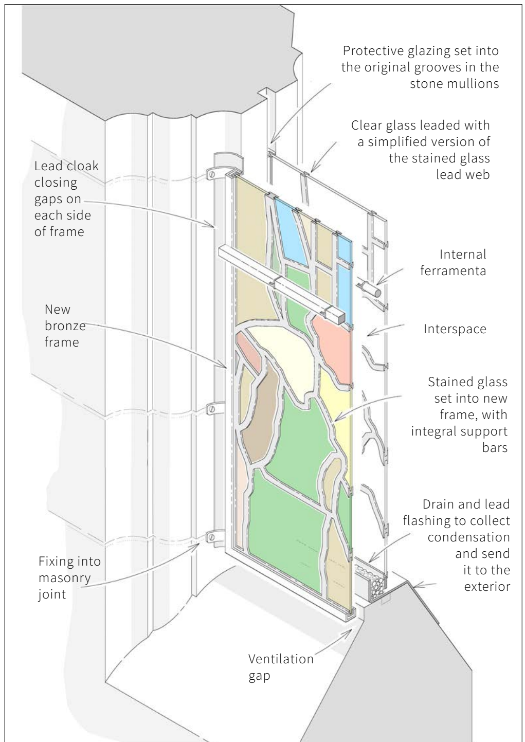
Figure 34 If the glass has been framed, a lead cloak can prevent halation.
