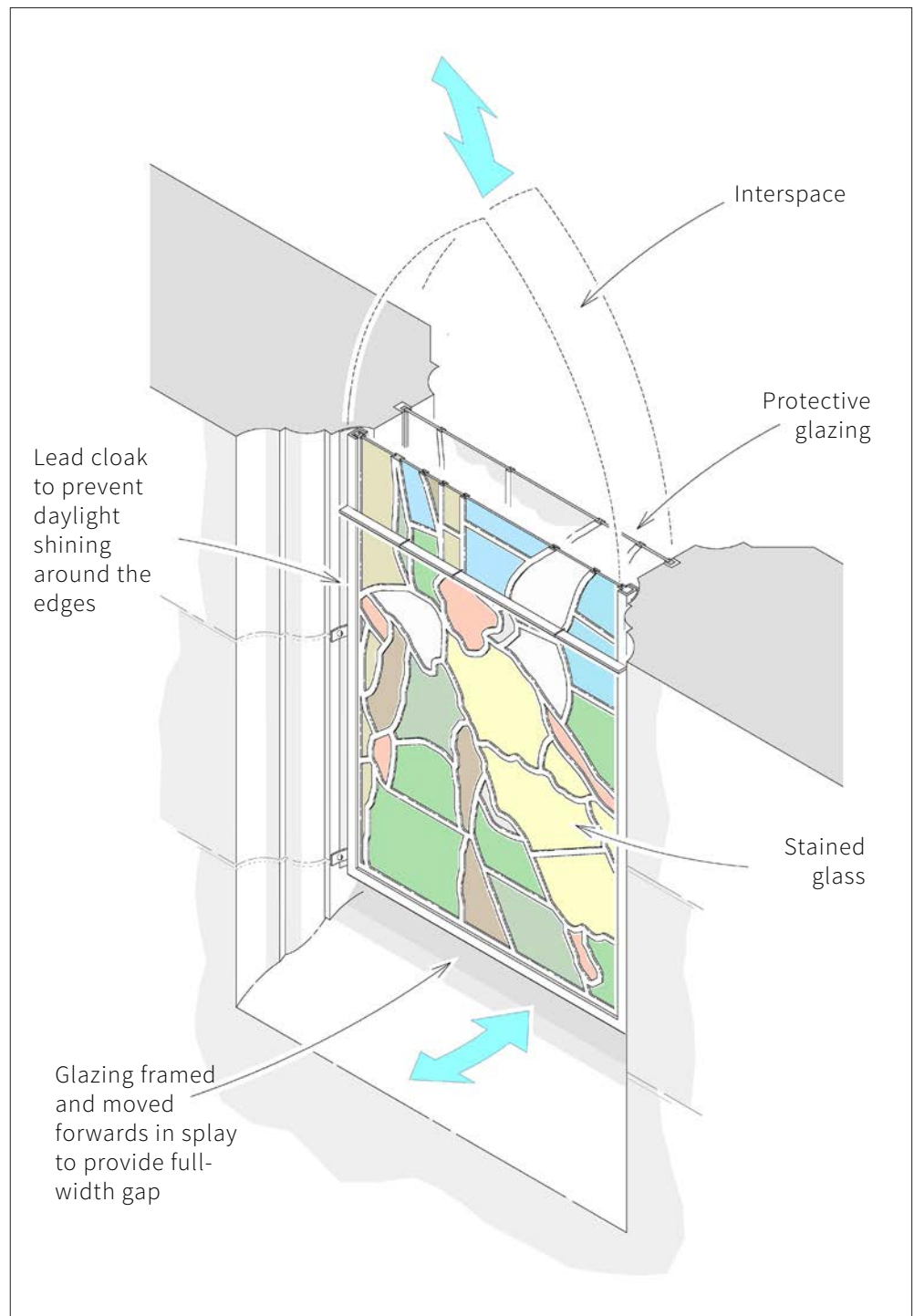
Figure 33 Options for ventilation The aim is to create smooth, laminar airflow through the interspace. This is best achieved by having a full-width opening at the bottom and top of the window. If the stained glass can be removed from its groove, one option is to set it into a metal frame and move it forwards into the interior, creating gaps around the glass that can be used to provide ventilation.
