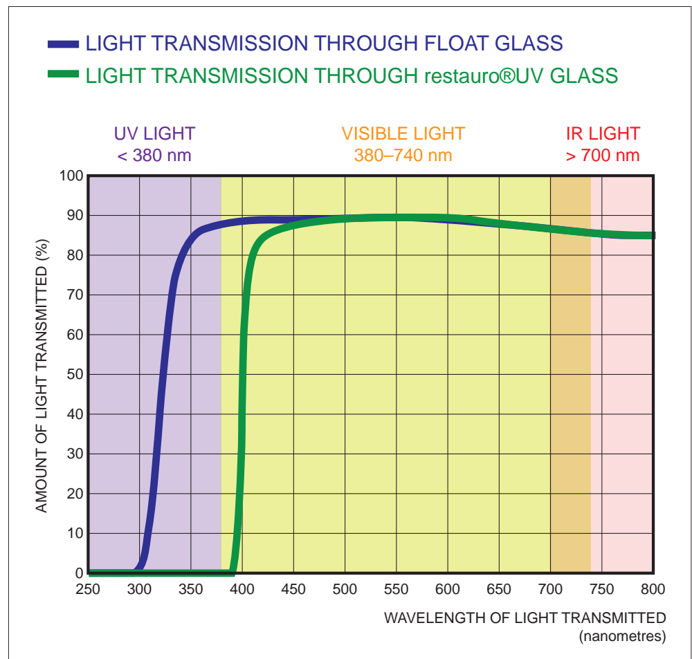
Figure 45 This graph compares the transmission of sunlight through float glass with its transmission through a specialist mouth-blown glass, which is able to filter out the UV component of sunlight reaching the original window. It is important to design filters so that they do not reduce too much of the incoming visible light, since this can affect the colours and intensity of the glass as seen from the interior.
