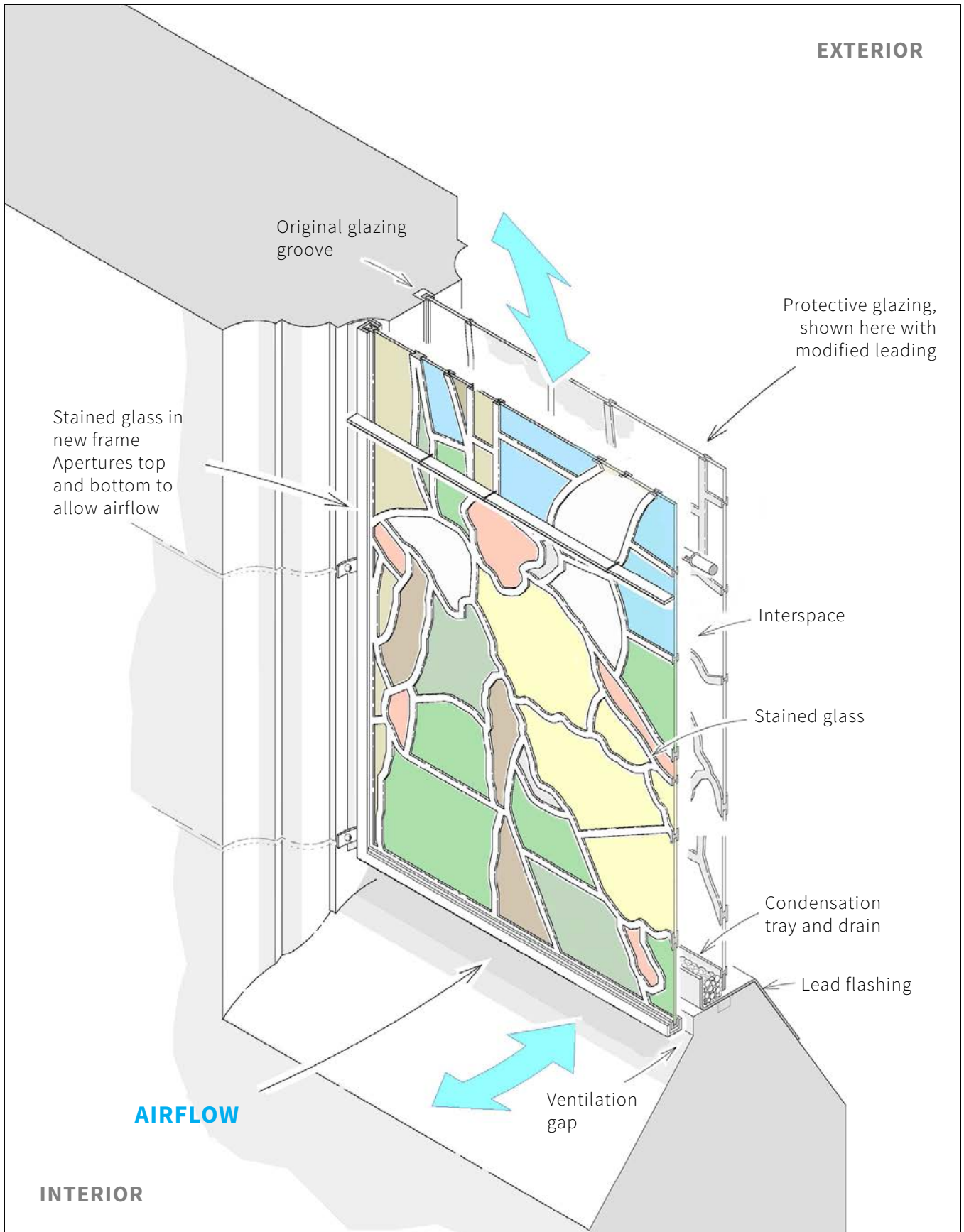
Figure 21 Basic elements of a typical internally ventilated EPG system The precise details of every EPG system will depend on the particular building and the configuration of the window being protected.
